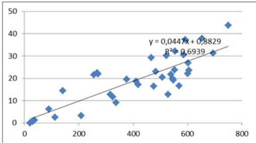
Fig.6. CHM and forest stand basal area
