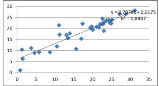
Fig.5. CHM and NFI sample plot average height data.
