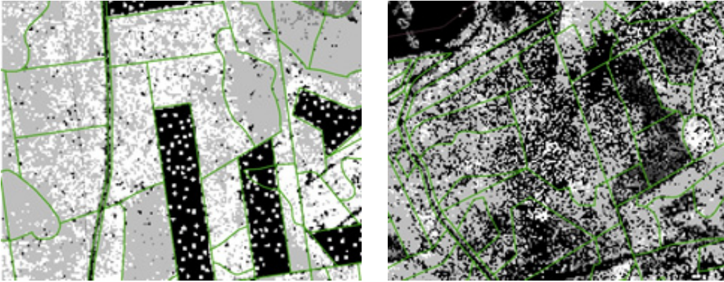
Fig.7. seed trees and scattered forest at CHM data.
