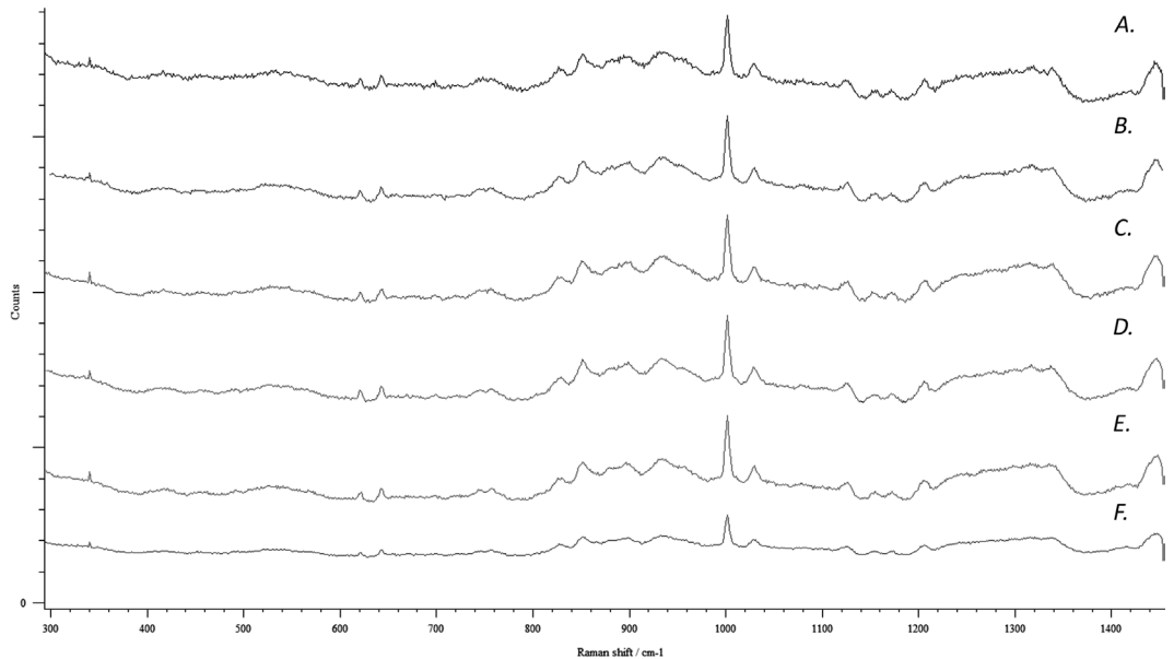
Fig. 2. Average Raman spectra of the unprocessed right-hand index fingertips skin epidermis of the 2 volunteers (in vitro). A,B,C- the man's skin samples D,E,F- the women's skin samples.
