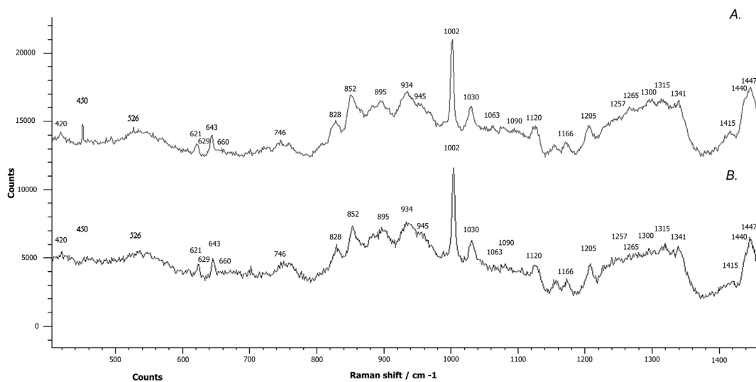
Fig.1. The estimates of pure Raman spectra: A. - the man's skin right-hand index fingertips epidermis, B. - the women's skin right-hand index fingertips epidermis, measured directly from the sample surface ( in vitro ).
