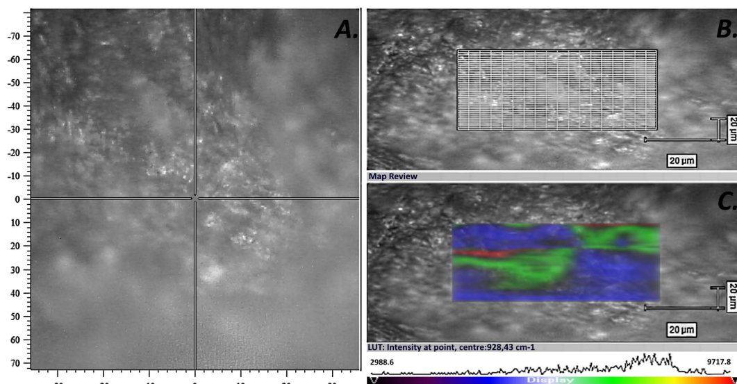
Fig. 3. Spatial 2D image of the human epidermis surface: A) an optical image; B) mapping scheme; C) micro-Raman signal intensity map.
